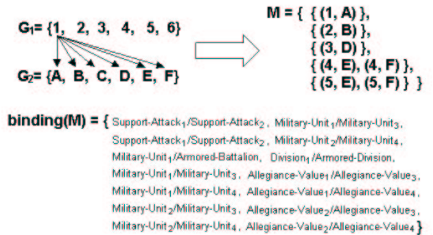
Figure 6: Illustration of Step 1.
