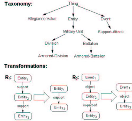
Figure 5: The taxonomy and transformations used in our example.
