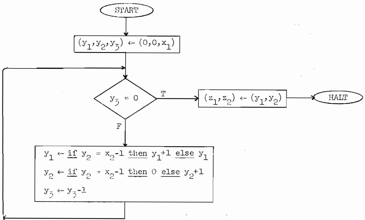
Figure 2: Another division program
