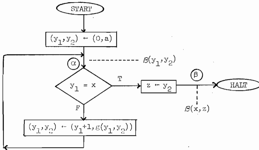
Figure 6: Labeled iterative 'going-up' program form
