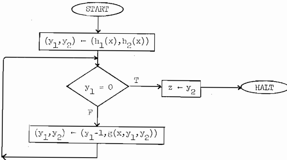
Figure 8: Iterative "going-down" program form
