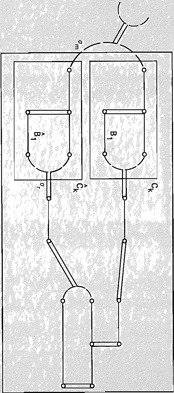
(a) G'_5
