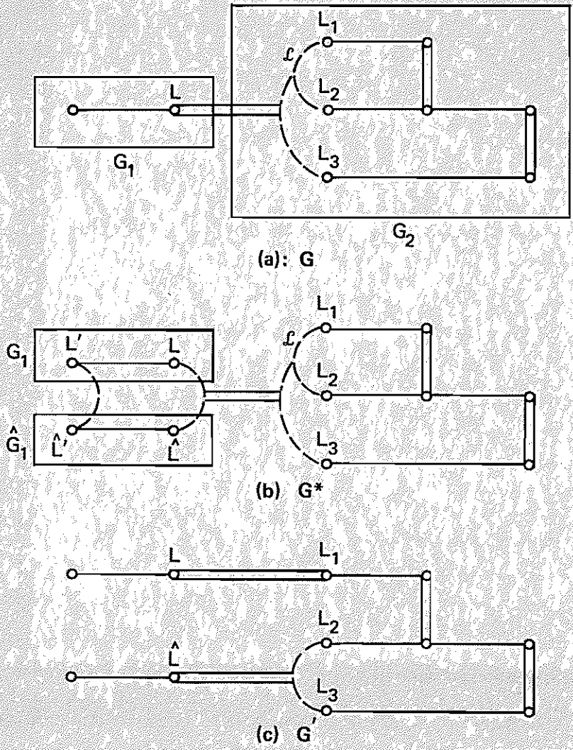
FIGURE 8 MERGE REDUCTION
