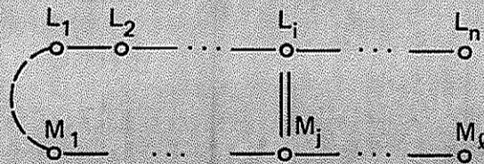
R(C, D)
