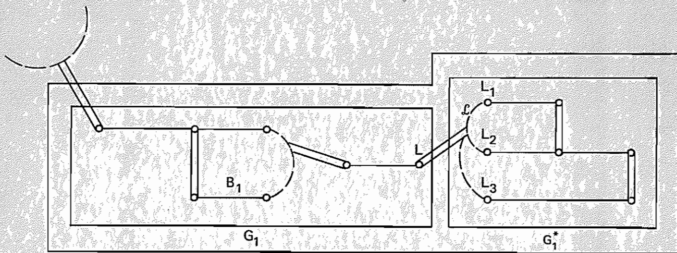
(a) G_5
