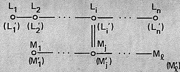
R(C, D)
