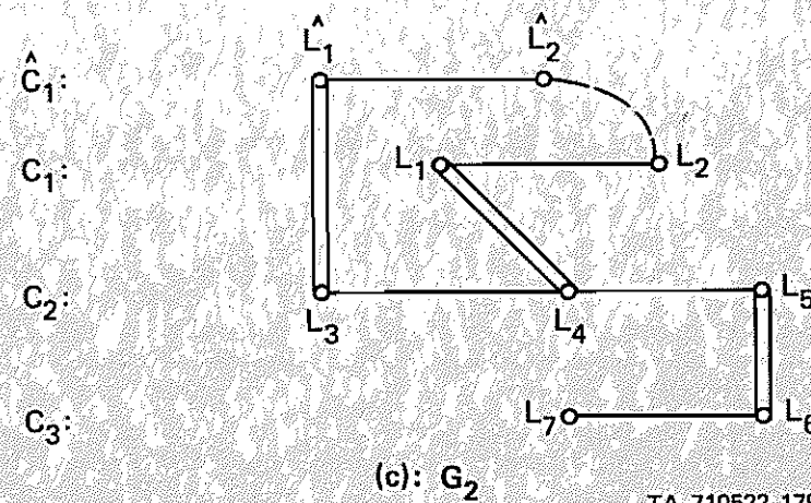
FIGURE 5 GRAPH DOMINANCE
