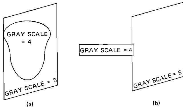
FIGURE 9 THE PHAGOCYTE HEURISTIC WILL FOR \theta_1 = 1/2 JOIN THE REGIONS OF (a) BUT NOT THOSE OF (b).
