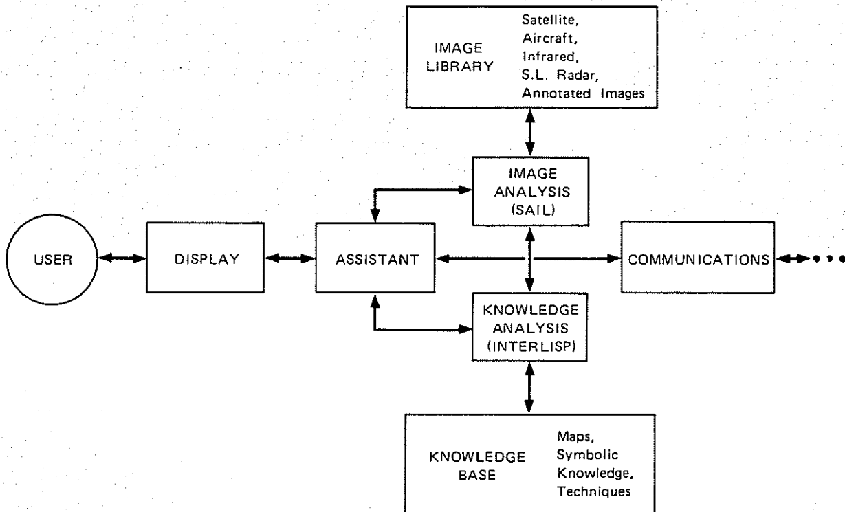
FIGURE 3 BLOCK DIAGRAM OF EXPERIMENTAL SYSTEM
