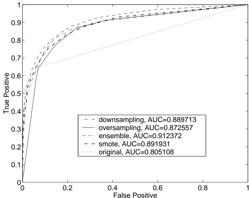
Fig. 4. ROC curves for the decision trees trained from different sampling approaches and the original training set.
