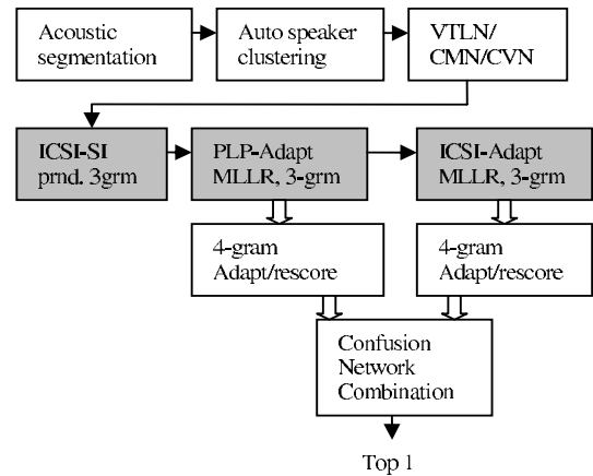
Fig. 2. System decoding architecture. Single arrows represent top 1 word sequence output, while block arrows represent top-n best word sequences.
