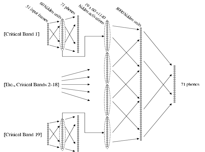
Fig. 1. The HATs feature, computed using a two-stage MLP. Notice the output from the hidden units of the first-stage MLPs is the input to the second-stage MLP.
