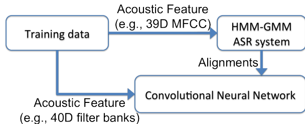
Figure 2: Flow diagram for CNN training for ASR.
