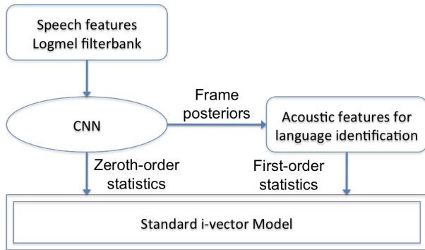
Figure 3: The flow diagram of CNN/i-vector hybrid system for i-vector model.
