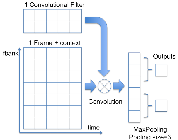
Figure 1: Diagram of a convolutional layer including convolution and max-pooling. Only one convolutional filter is shown in this example and non-overlapping pooling is used.
