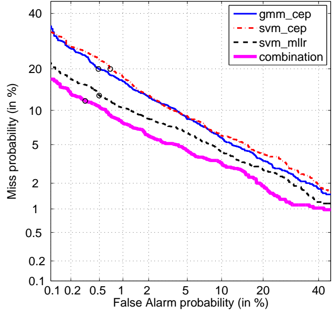
Fig. 2. Detection error tradeoff (DET) curves for baseline, 8+8-transform MLLR, and combined systems, SRE-05 1-conversation-side condition.
