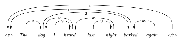
Figure 1. A Sentence S and its Linkage K . \langle s \rangle and \langle /s \rangle are sentence delimiters.
